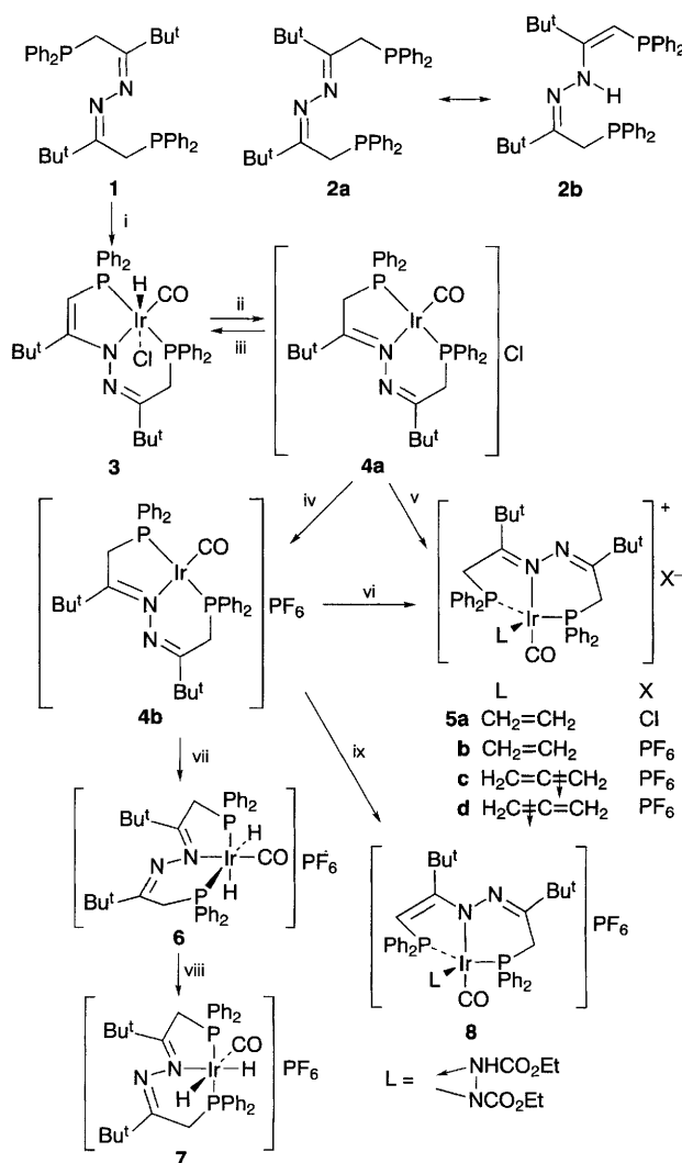
Scheme 1 Reagents and conditions: i, [\text{IrCl}(\text{CO})_2(p\text{-toluidine})] ; ii, EtOH or MeOH; iii, \text{C}_6\text{H}_6 or \text{CH}_2\text{Cl}_2 ; iv, \text{NH}_4\text{PF}_6 ; v, L or L/ \text{NH}_4\text{PF}_6 ; vi, for 5b - 5d , L; vii, H 2 ; viii, 20 °C, 24 h; ix, \text{EtO}_2\text{CN}=\text{NCO}_2\text{Et}
